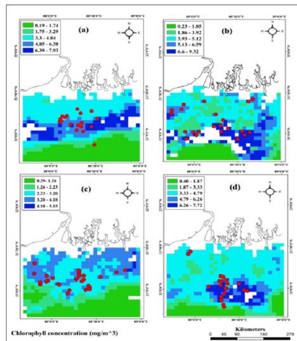
Fig. 2—The plots of high fish catch locations along with the spatial extent of chlorophyll variability for the months of (a) October' 2012 (b) October' 2013 (c) November' 2012 (d) November' 2013.
