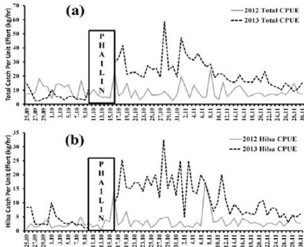
Fig. 3—The trend of (a) total CPUE and (b) Hilsa CPUE before and after the cyclone Phailin in the year 2013 along with the corresponding CPUE of the same time period in the year 2012.
