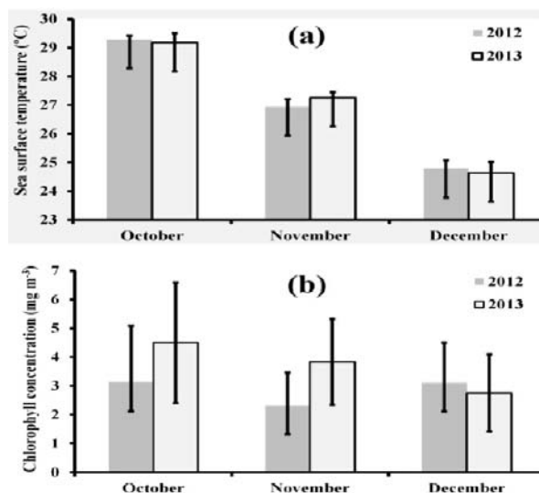
Fig. 1—Monthly mean (a) SST and (b) chlorophyll concentration for the months of October, November and December in both the years 2012 and 2013. The error bars denoting the standard deviation.
